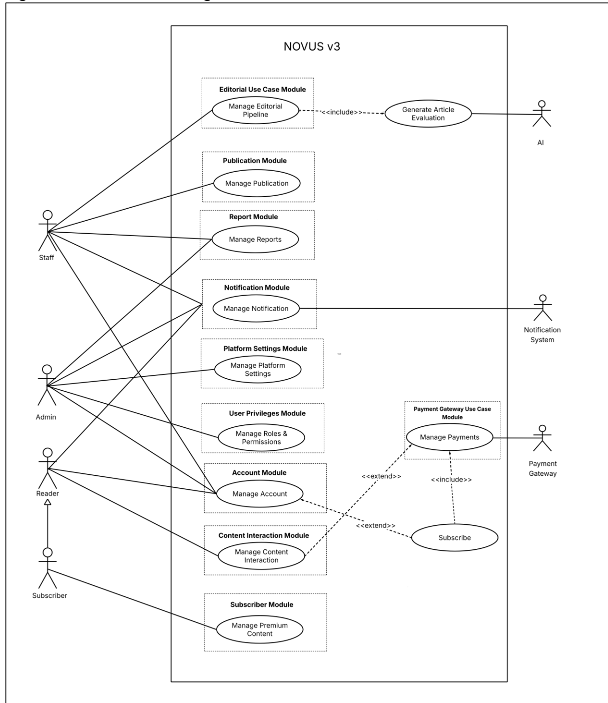
Figure 1. NOVUS Use Case Diagram
