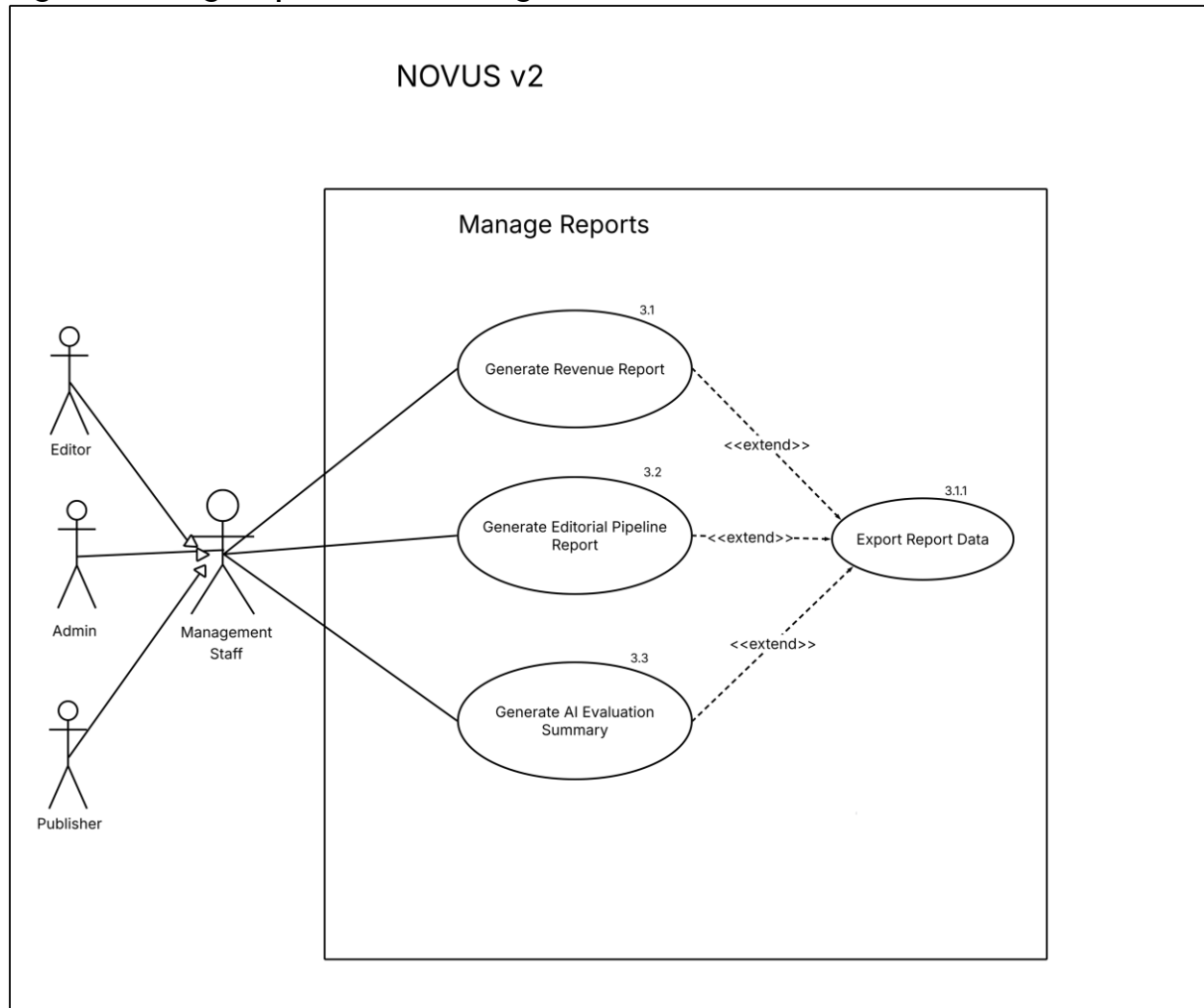
Figure 4. Manage Reports Use Case Diagram
