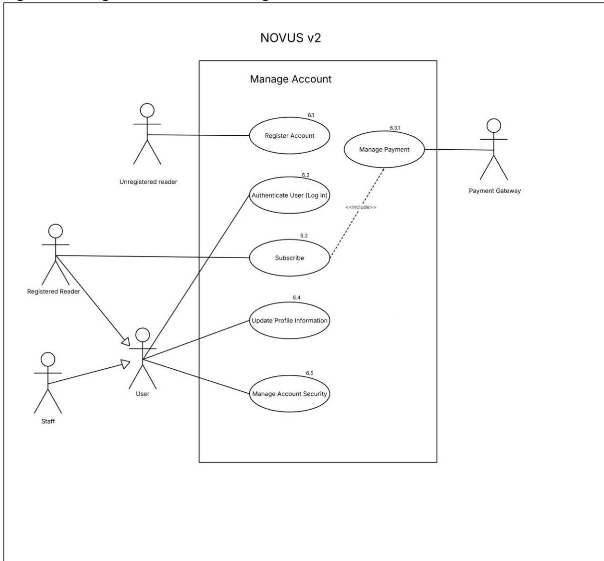
Figure 7. Manage Account Use Case Diagram
