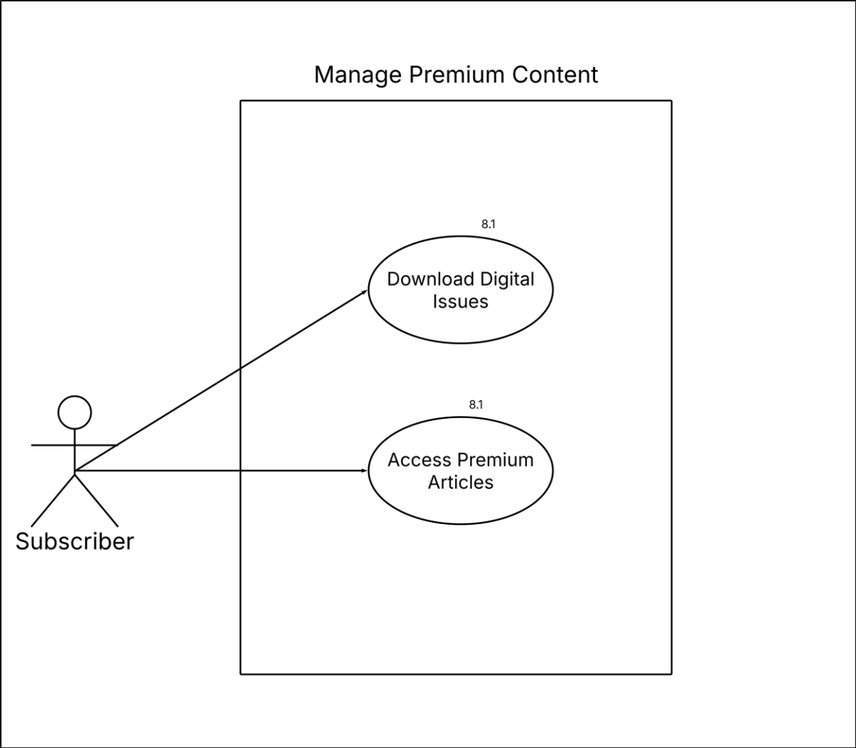
Figure 9. Manage Premium Content Use Case Diagram
