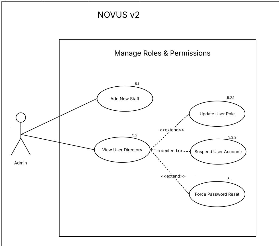
Figure 6. Manage User Privileges Use Case Diagram
